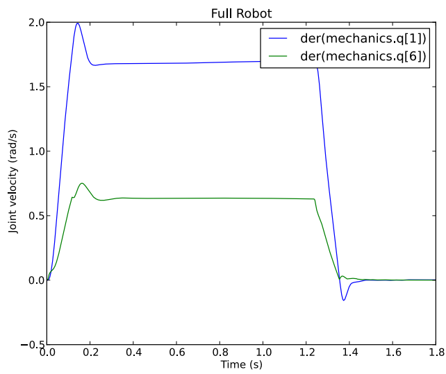
Figure 7.11. Comparison with Dymola
