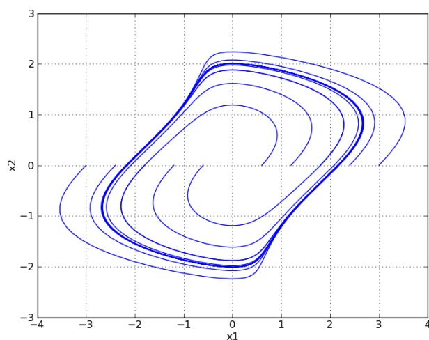
Figure 7.7. Simulation result-phase plane
